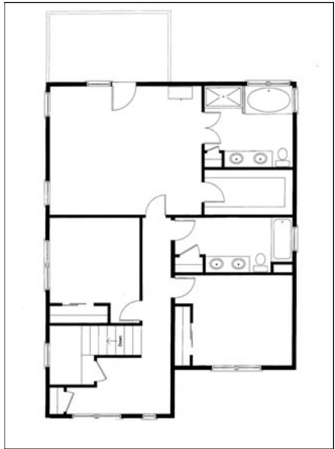
Second Floor
